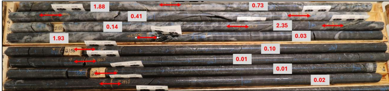
Figure 3: Quartz Vein Zone in GR-25-012 with Assays in g/t Au.
