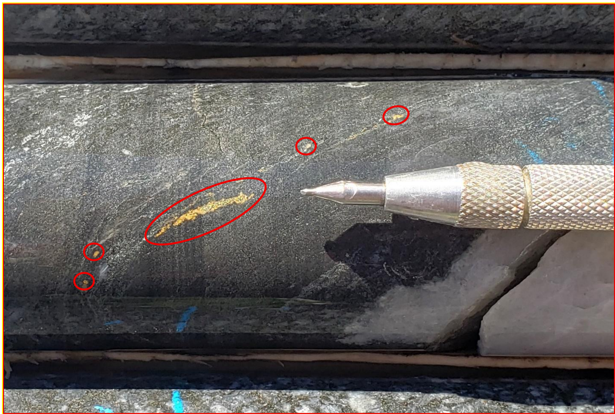
Figure 2: Visible Gold in the Interval 11.8-12.1 m, Hole GR-25-011 Which Assayed 308 g/t Au 3
