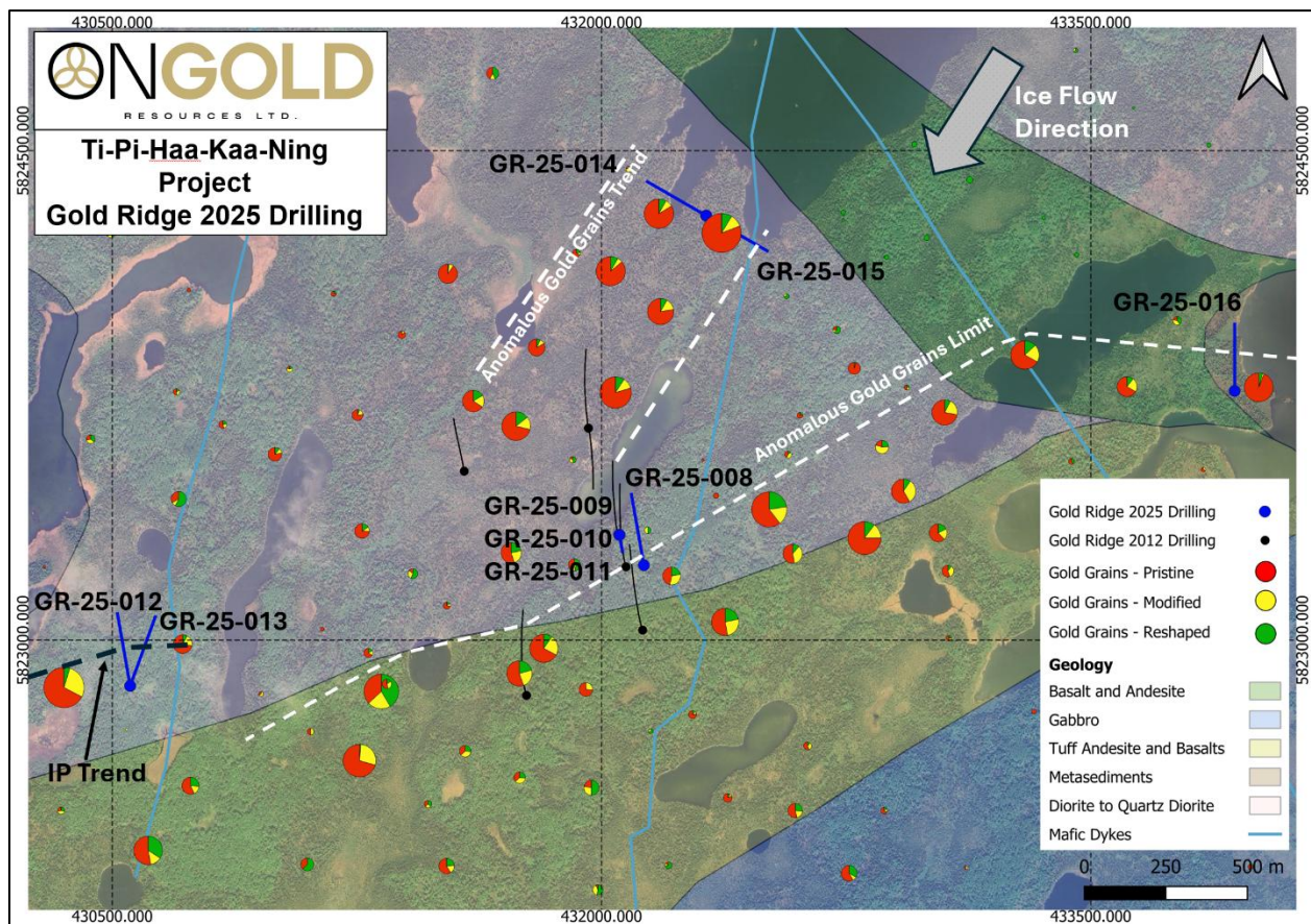
Figure 1 : Historical gold grains-in-till results, interpreted geology, historical and recent drilling, Gold Ridge area.
